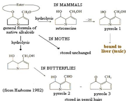
Figure 2. Mechanism of transformation of Pyrrolizidine alkaloids
